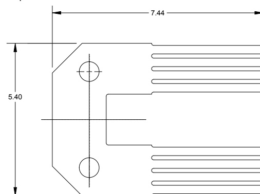
Wiper 2
